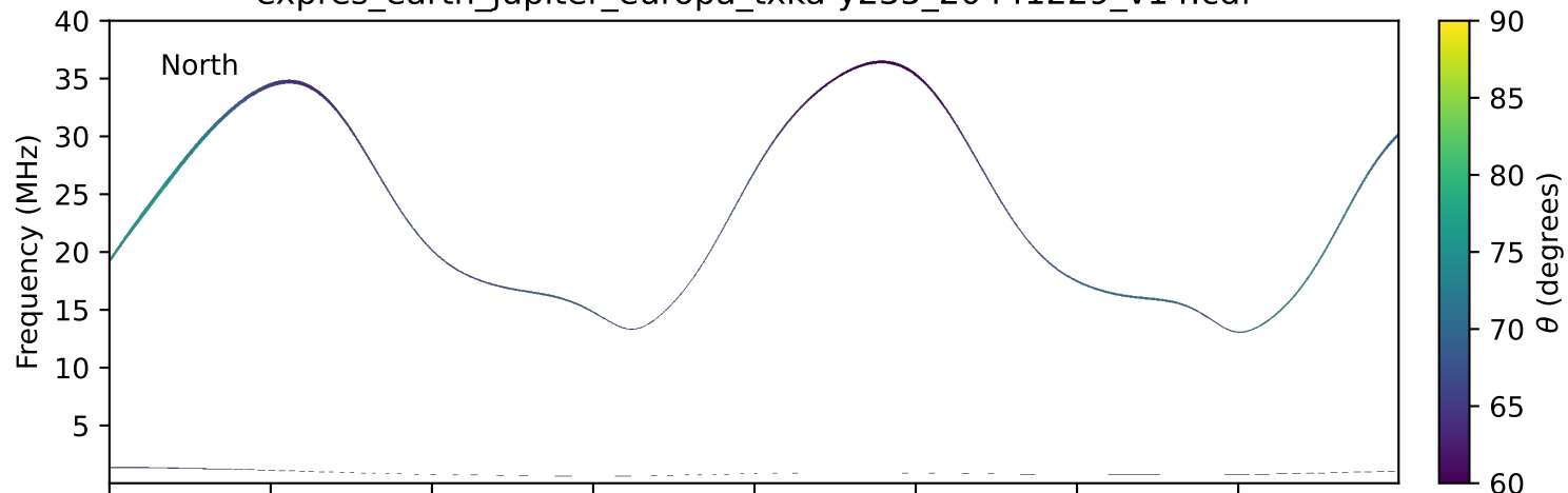
expres_earth_jupiter_europa_txka-y235_20441229_v14.cdf
