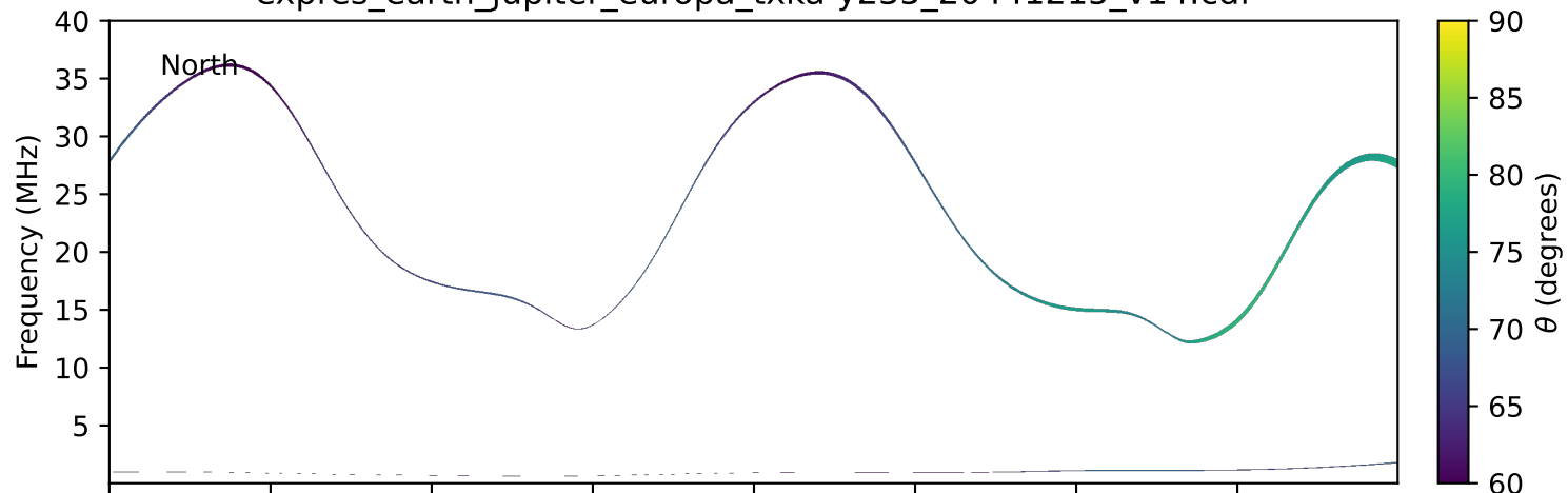
expres_earth_jupiter_europa_txka-y235_20441215_v14.cdf
