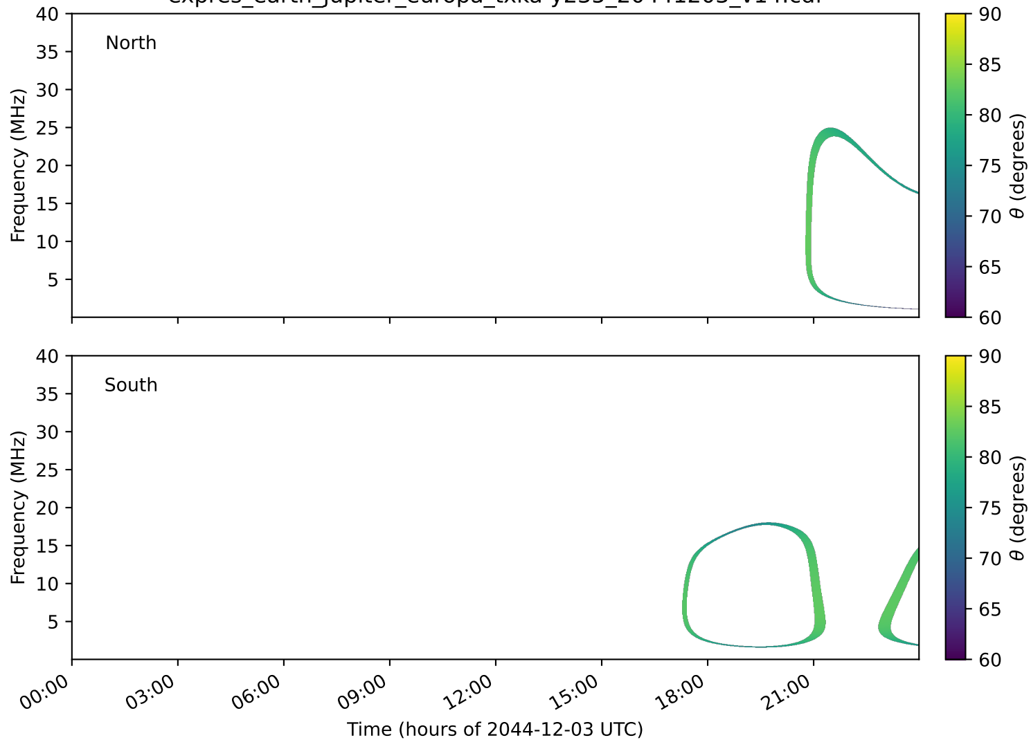
expres_earth_jupiter_europa_txka-y235_20441203_v14.cdf
