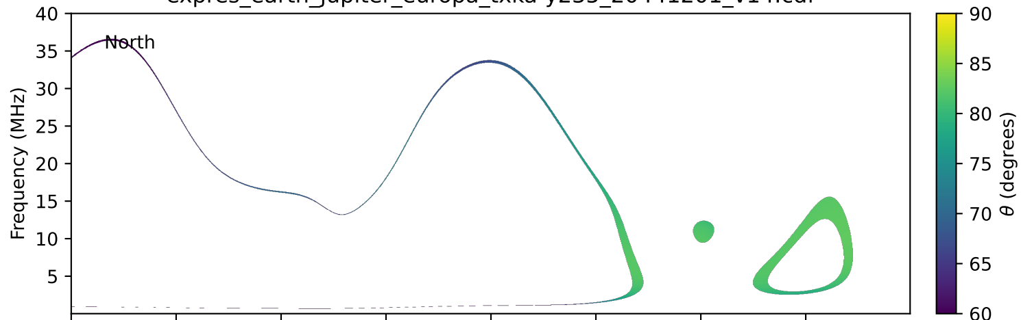
expres_earth_jupiter_europa_txka-y235_20441201_v14.cdf
