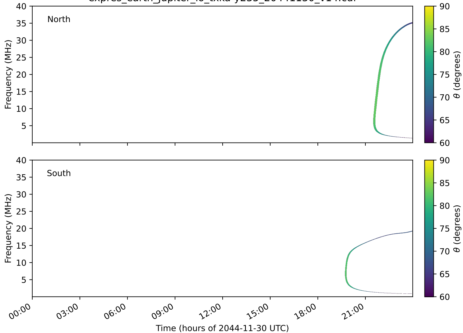
expres_earth_jupiter_io_txka-y235_20441130_v14.cdf
