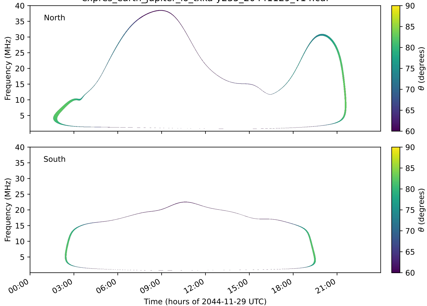
expres_earth_jupiter_io_txka-y235_20441129_v14.cdf
