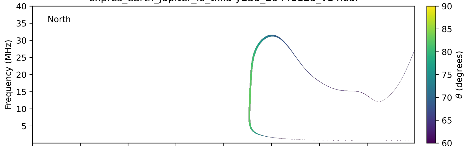
expres_earth_jupiter_io_txka-y235_20441125_v14.cdf
