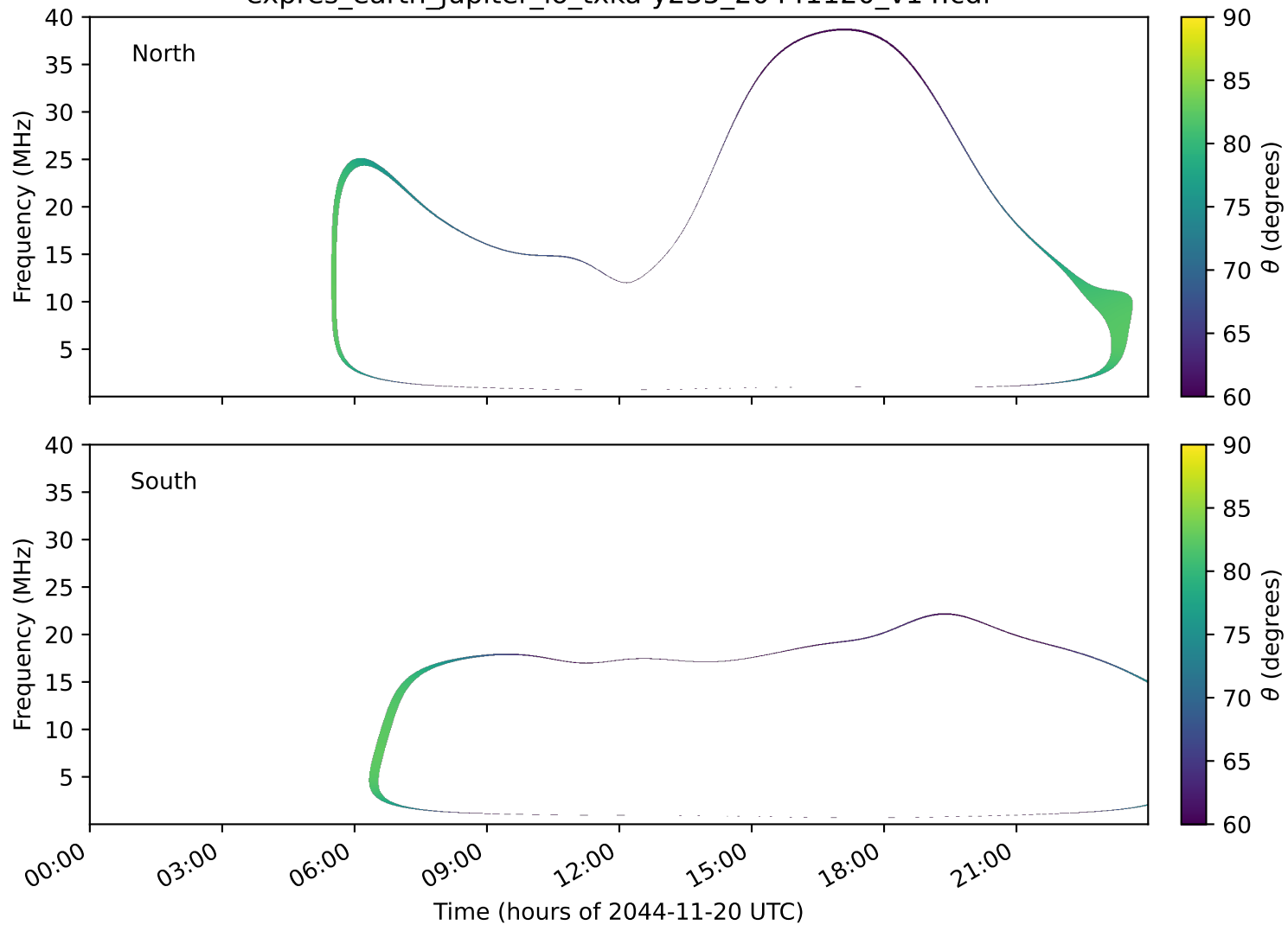
expres_earth_jupiter_io_txka-y235_20441120_v14.cdf
