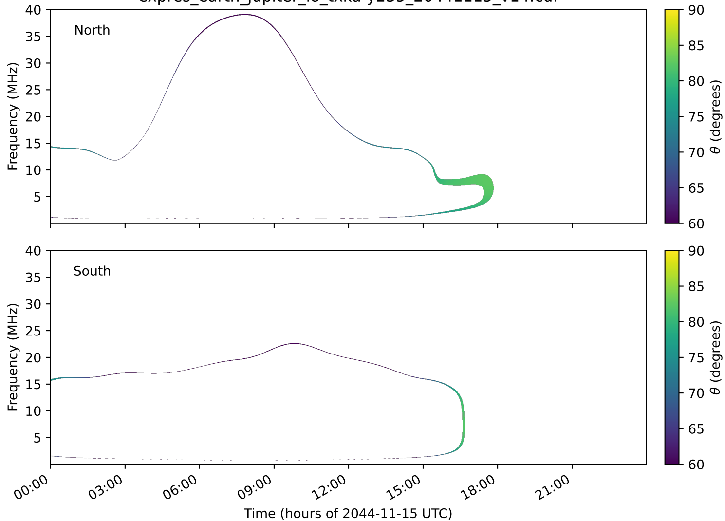
expres_earth_jupiter_io_txka-y235_20441115_v14.cdf
