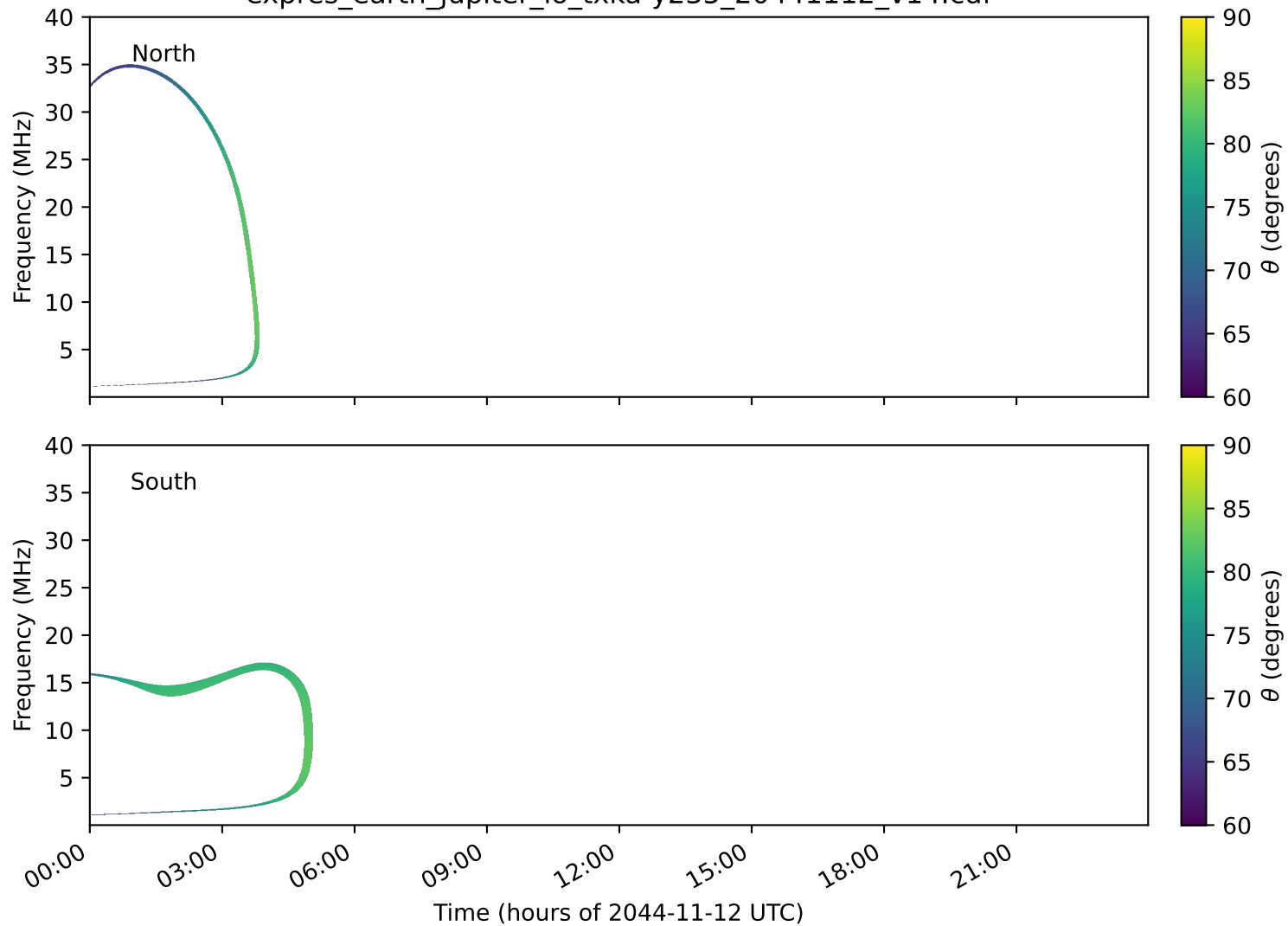
expres_earth_jupiter_io_txka-y235_20441112_v14.cdf
