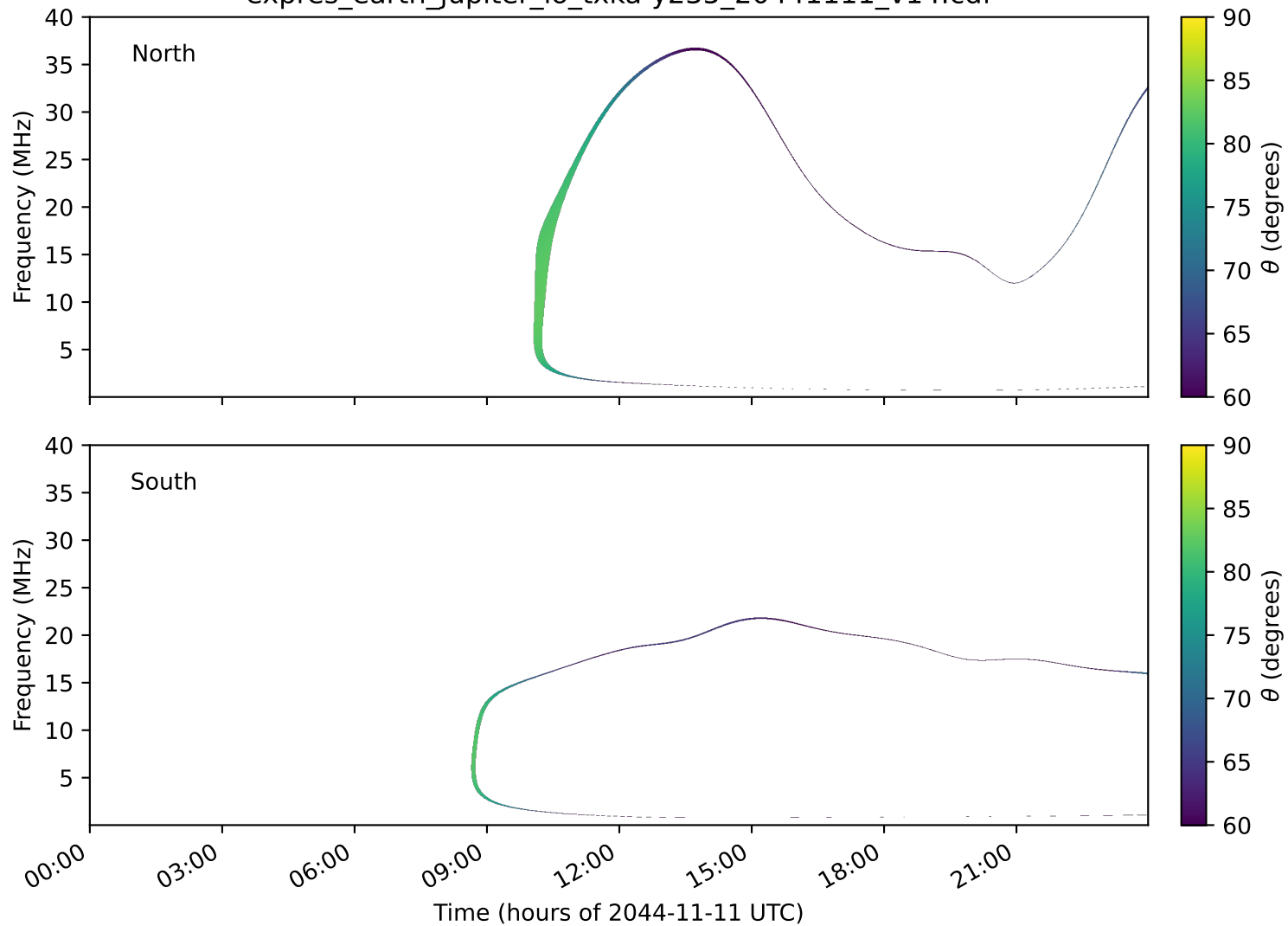
expres_earth_jupiter_io_txka-y235_20441111_v14.cdf
