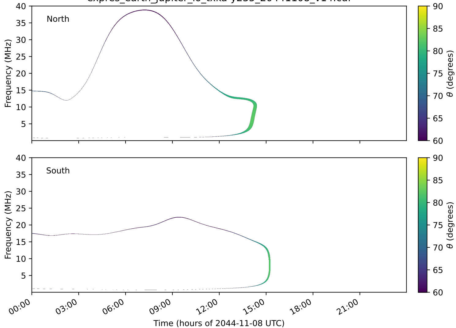
expres_earth_jupiter_io_txka-y235_20441108_v14.cdf
