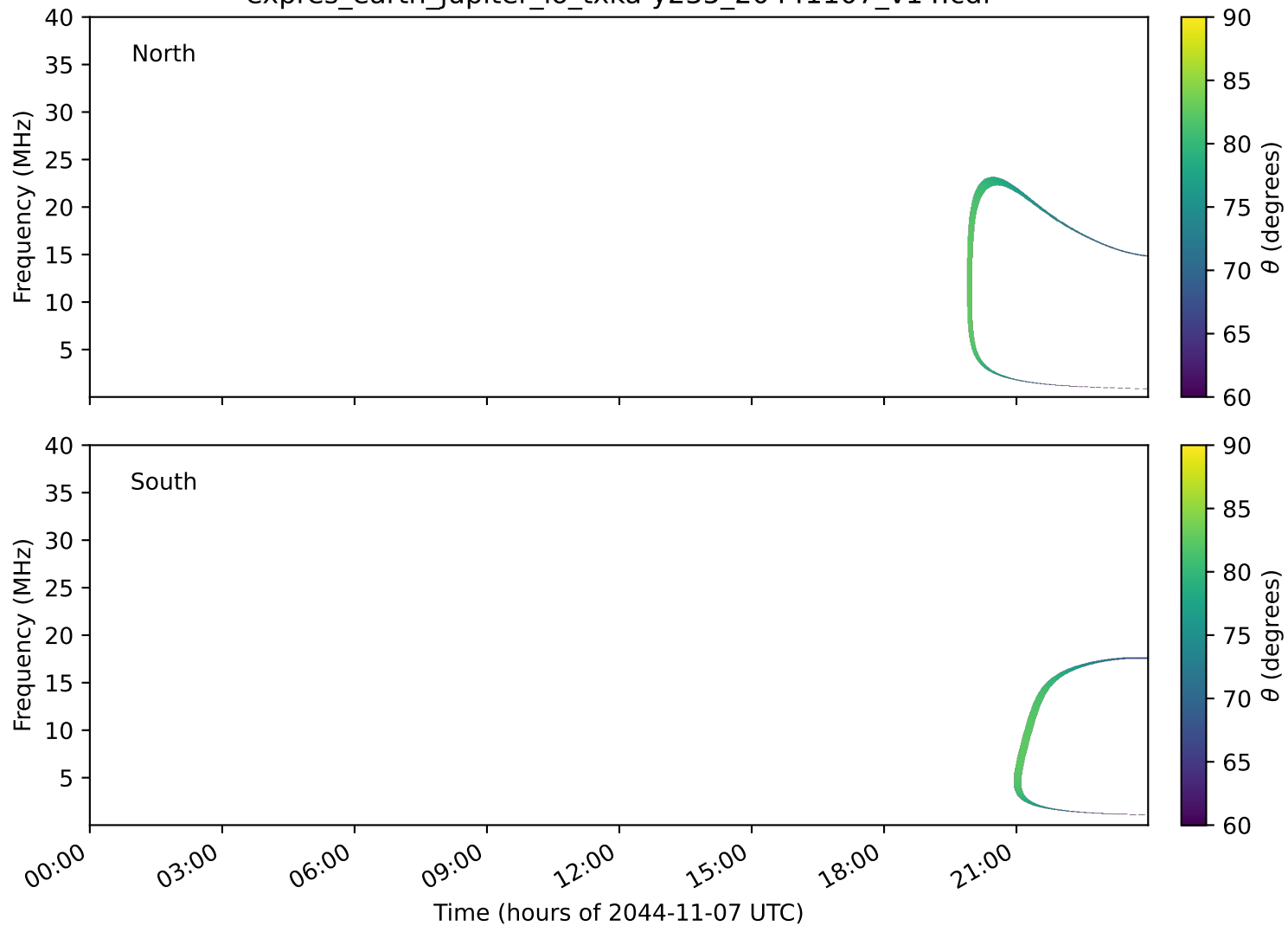
expres_earth_jupiter_io_txka-y235_20441107_v14.cdf
