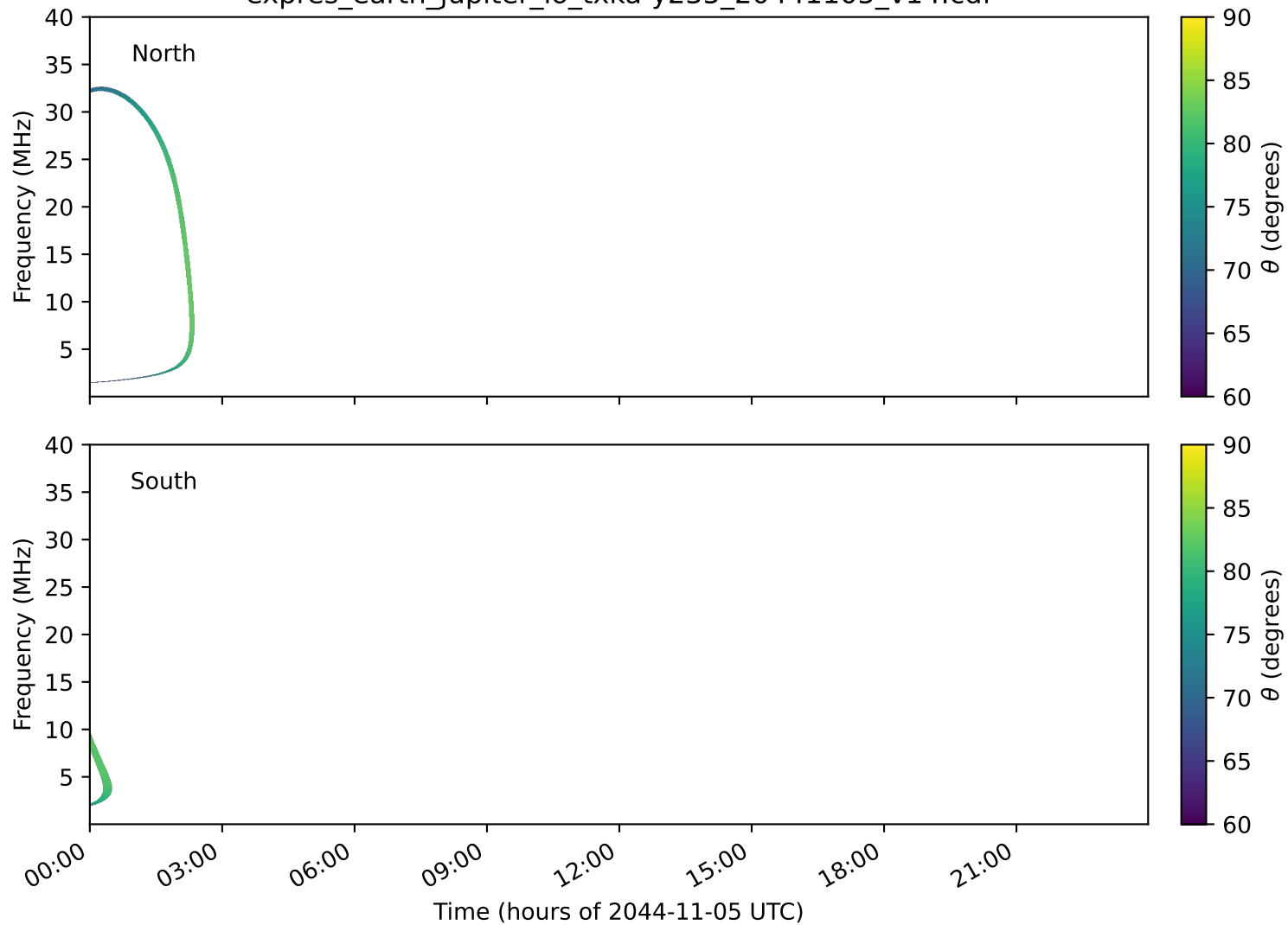
expres_earth_jupiter_io_txka-y235_20441105_v14.cdf
