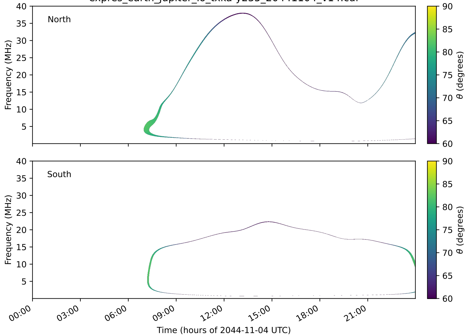
expres_earth_jupiter_io_txka-y235_20441104_v14.cdf
