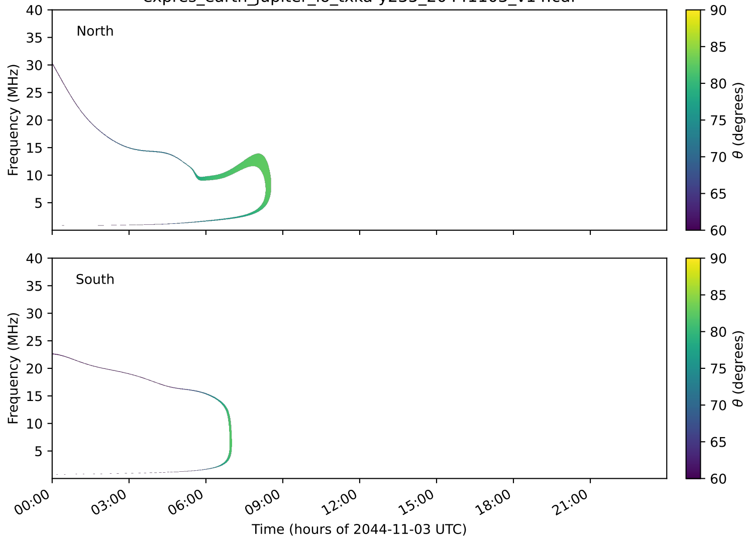
expres_earth_jupiter_io_txka-y235_20441103_v14.cdf
