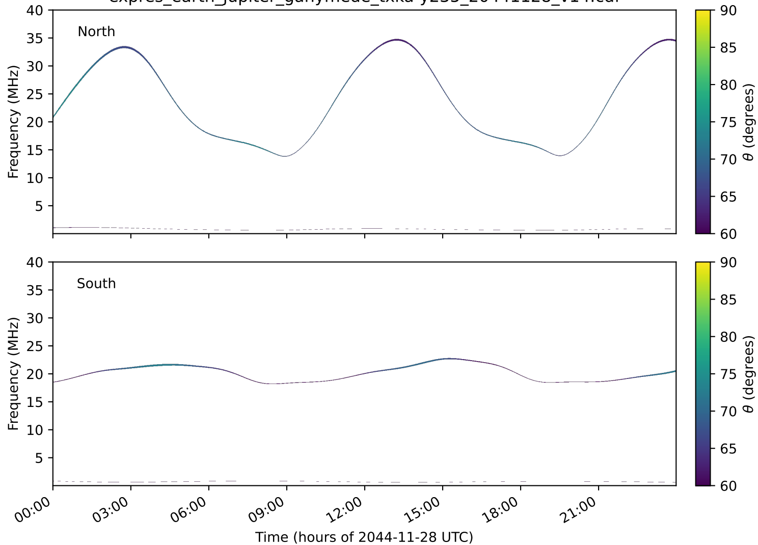
expres_earth_jupiter_ganymede_txka-y235_20441128_v14.cdf
