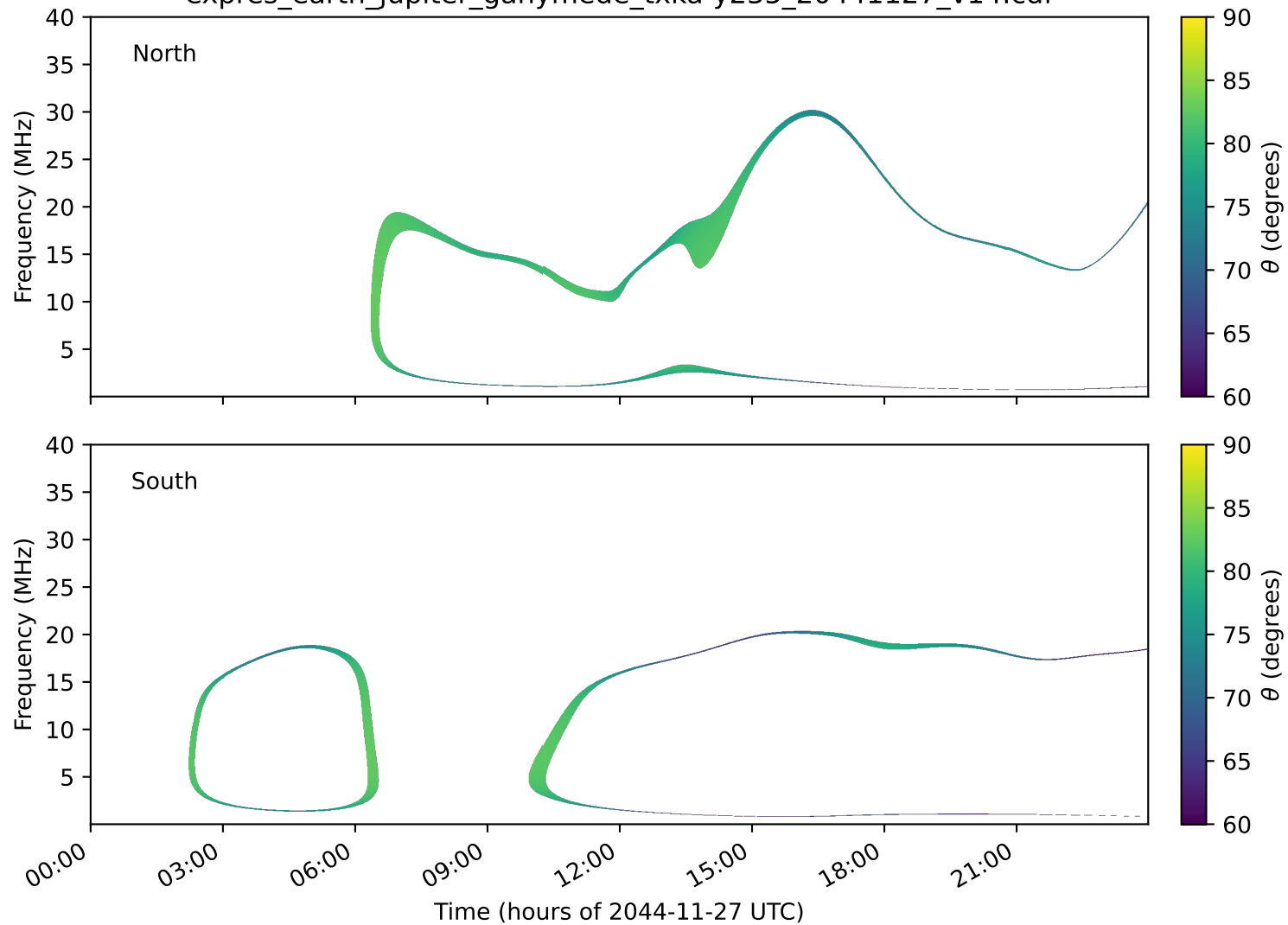
expres_earth_jupiter_ganymede_txka-y235_20441127_v14.cdf
