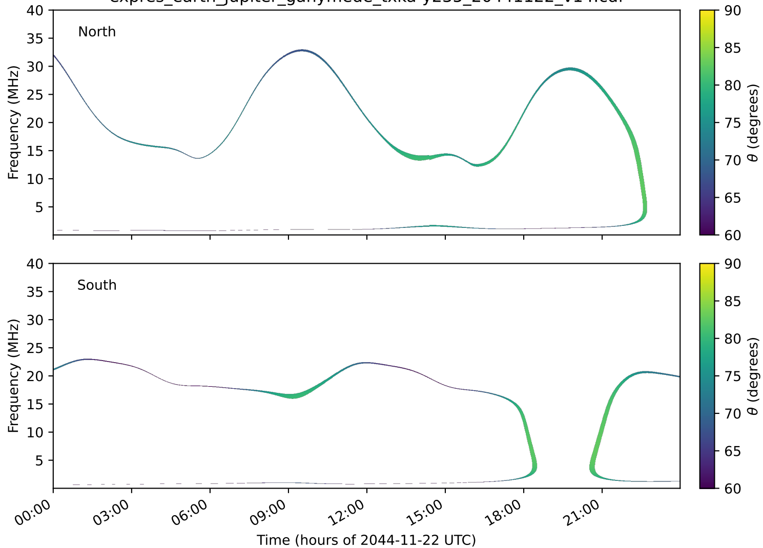
expres_earth_jupiter_ganymede_txka-y235_20441122_v14.cdf
