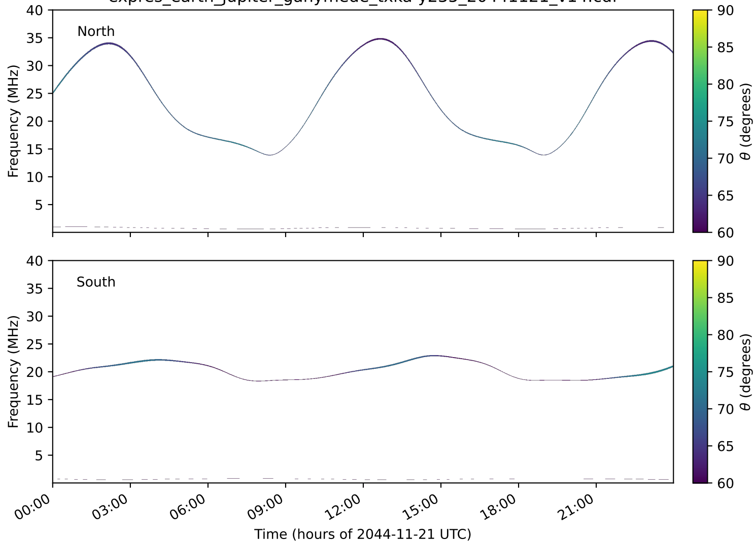
expres_earth_jupiter_ganymede_txka-y235_20441121_v14.cdf
