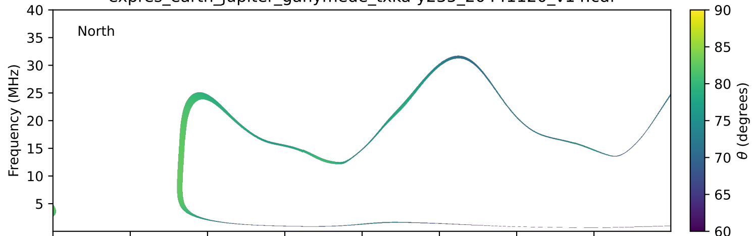
expres_earth_jupiter_ganymede_txka-y235_20441120_v14.cdf
