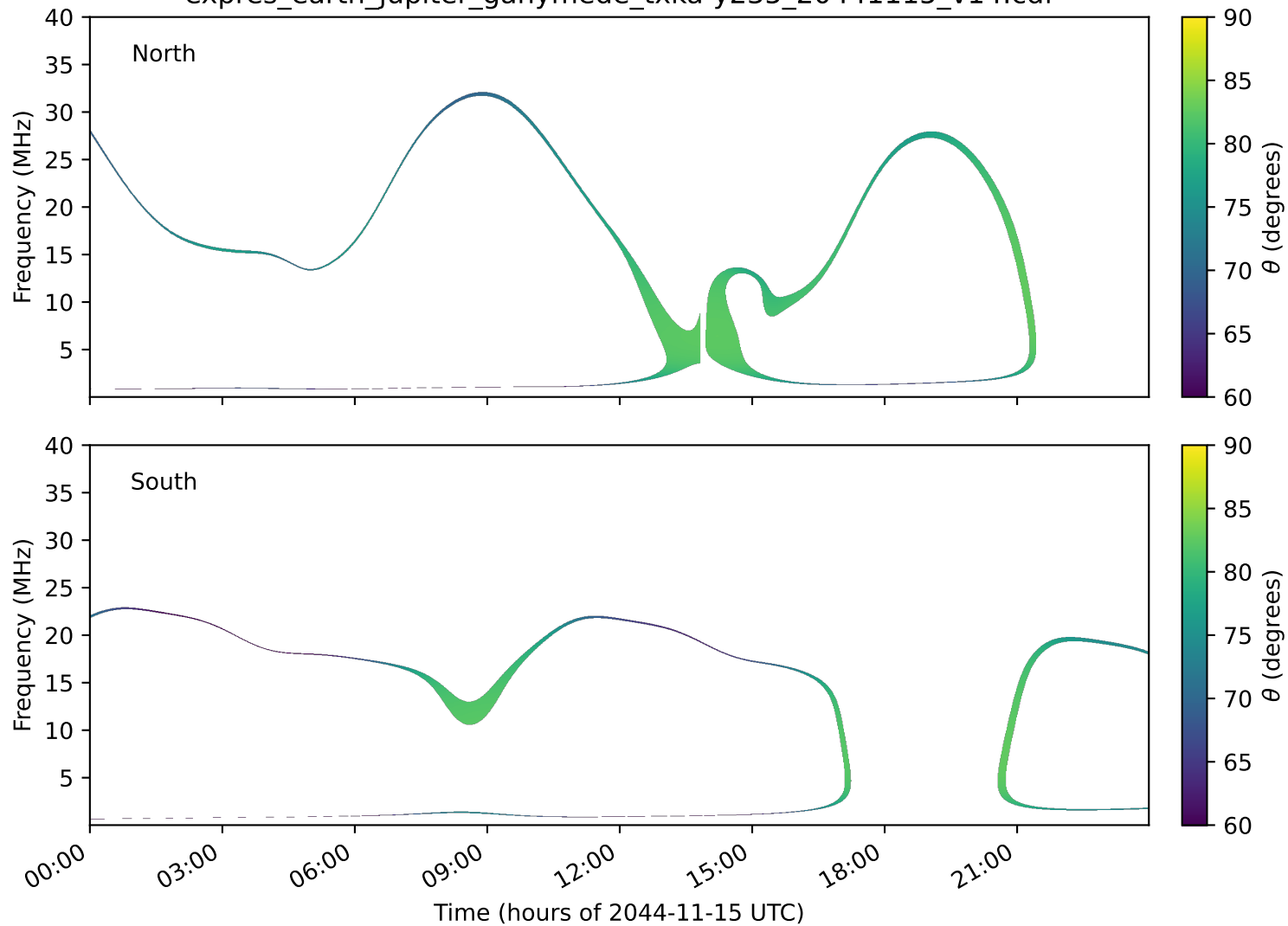
expres_earth_jupiter_ganymede_txka-y235_20441115_v14.cdf
