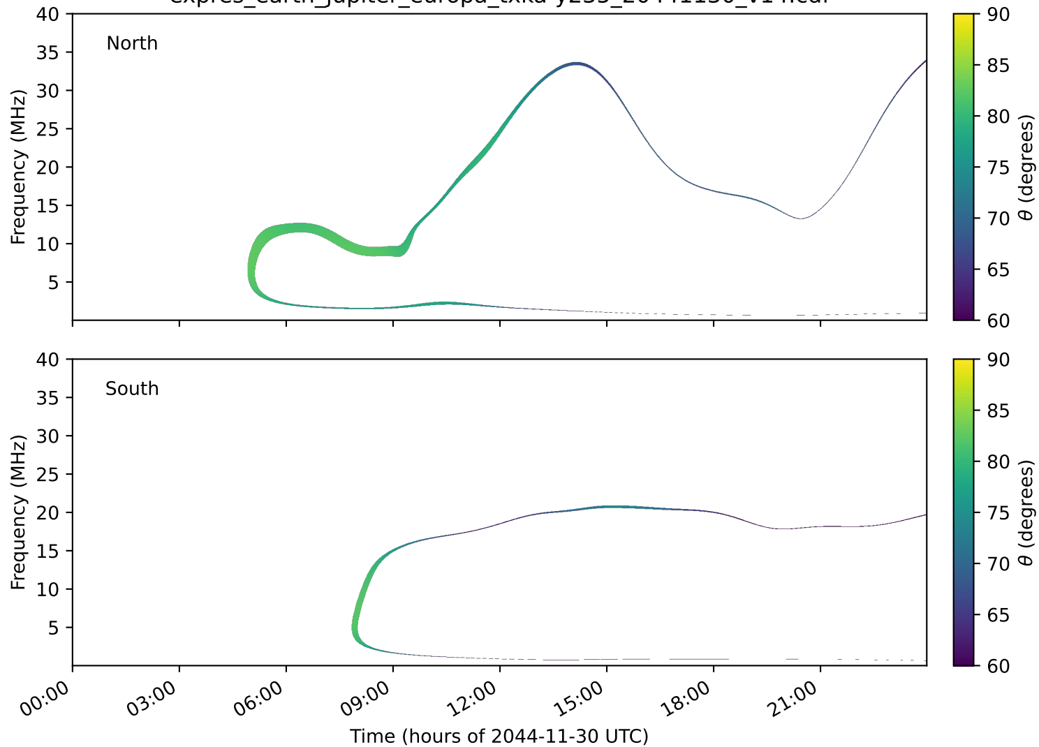
expres_earth_jupiter_europa_txka-y235_20441130_v14.cdf
