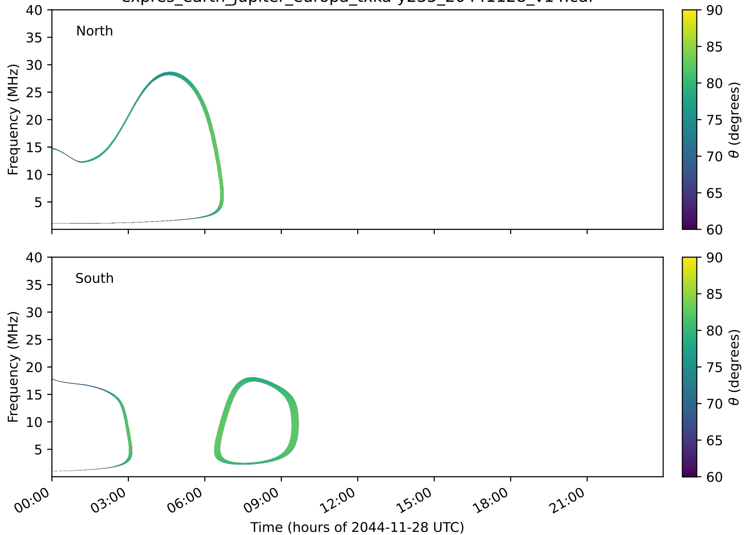
expres_earth_jupiter_europa_txka-y235_20441128_v14.cdf
