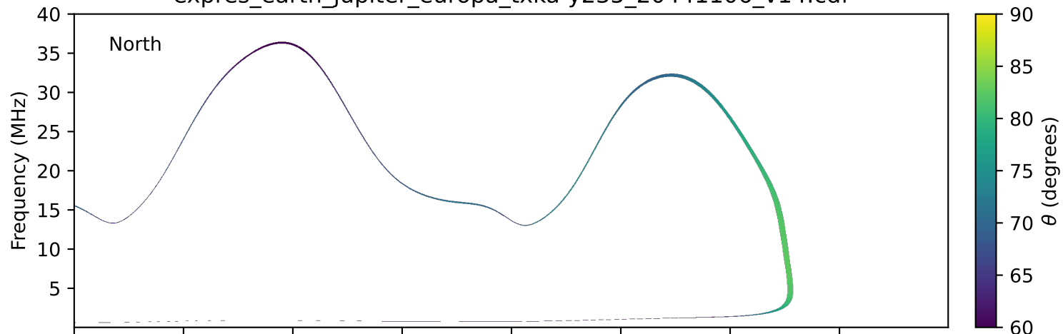
expres_earth_jupiter_europa_txka-y235_20441106_v14.cdf
