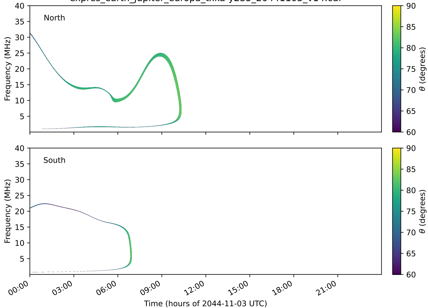
expres_earth_jupiter_europa_txka-y235_20441103_v14.cdf
