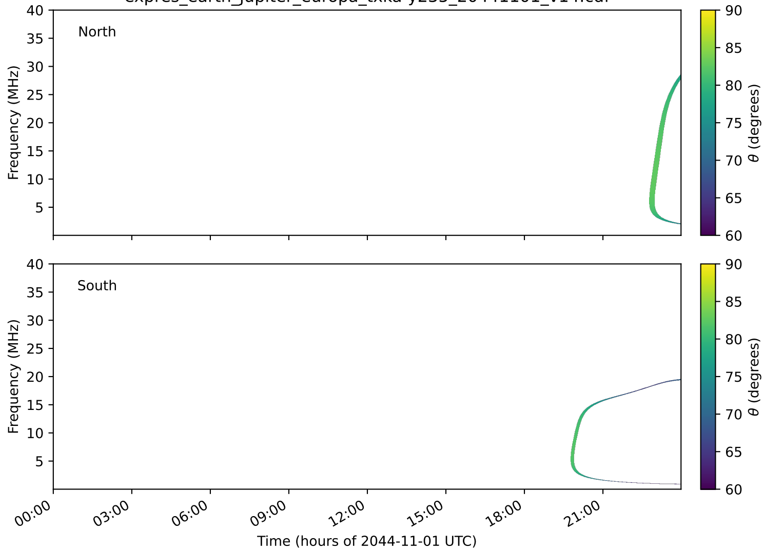
expres_earth_jupiter_europa_txka-y235_20441101_v14.cdf
