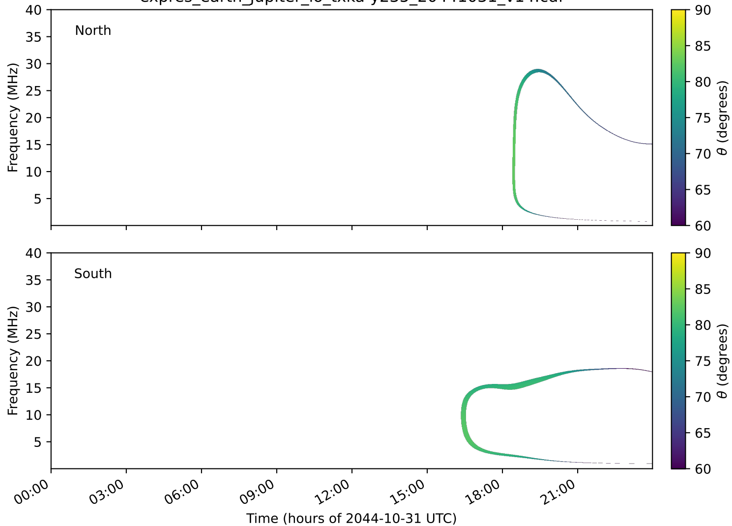
expres_earth_jupiter_io_txka-y235_20441031_v14.cdf
