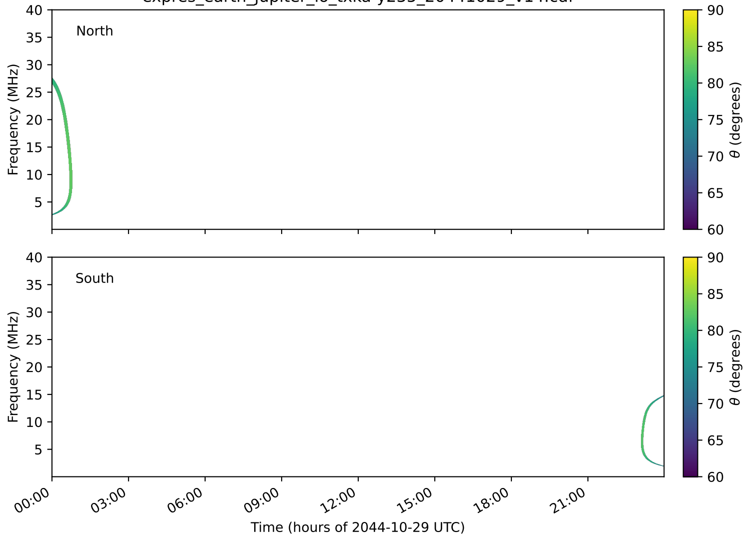
expres_earth_jupiter_io_txka-y235_20441029_v14.cdf
