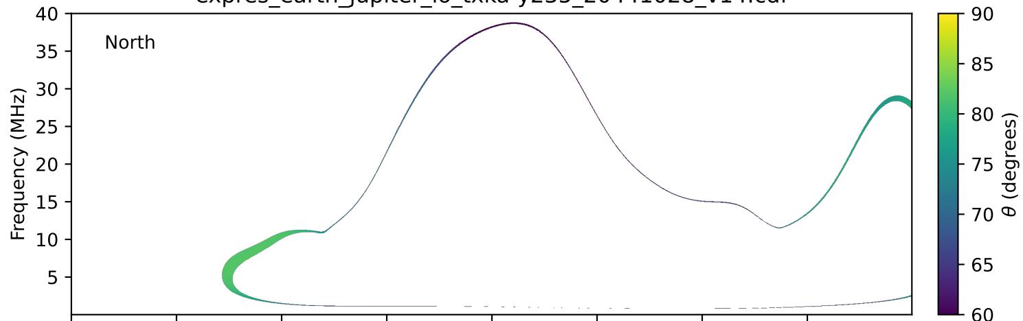
expres_earth_jupiter_io_txka-y235_20441028_v14.cdf
