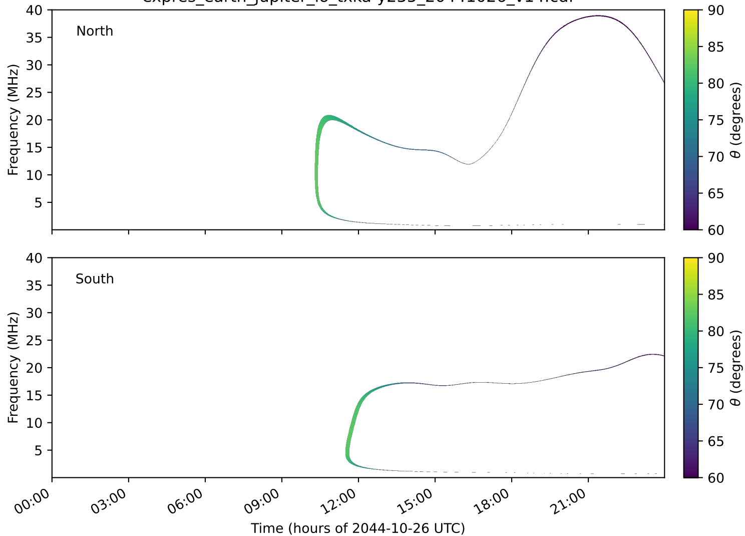
expres_earth_jupiter_io_txka-y235_20441026_v14.cdf
