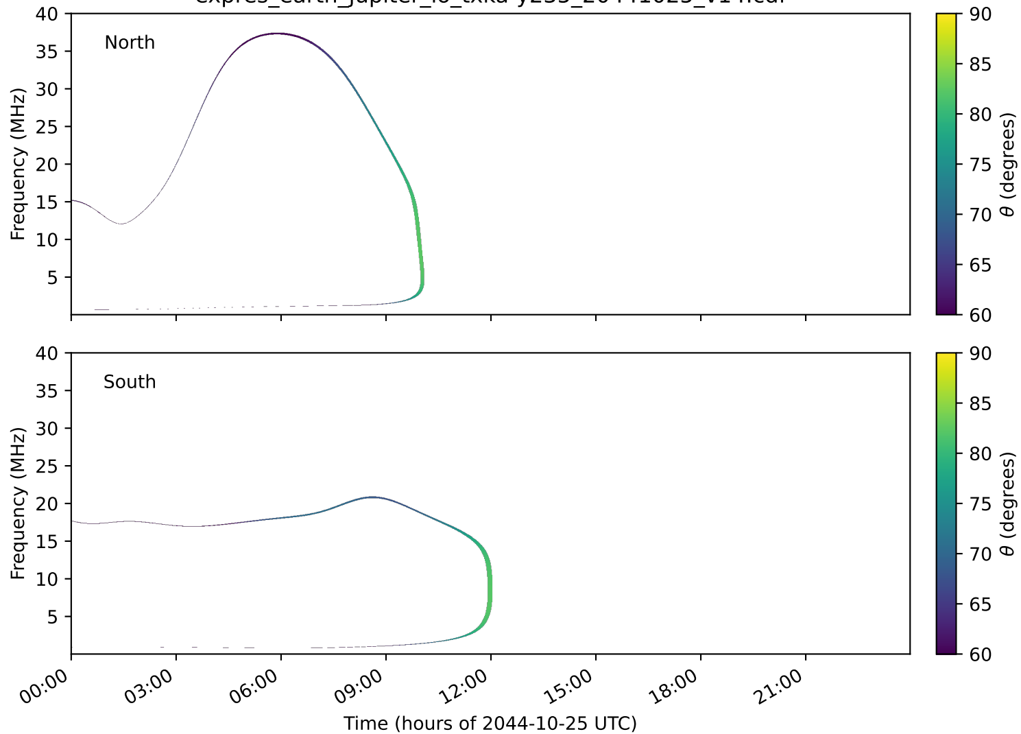
expres_earth_jupiter_io_txka-y235_20441025_v14.cdf
