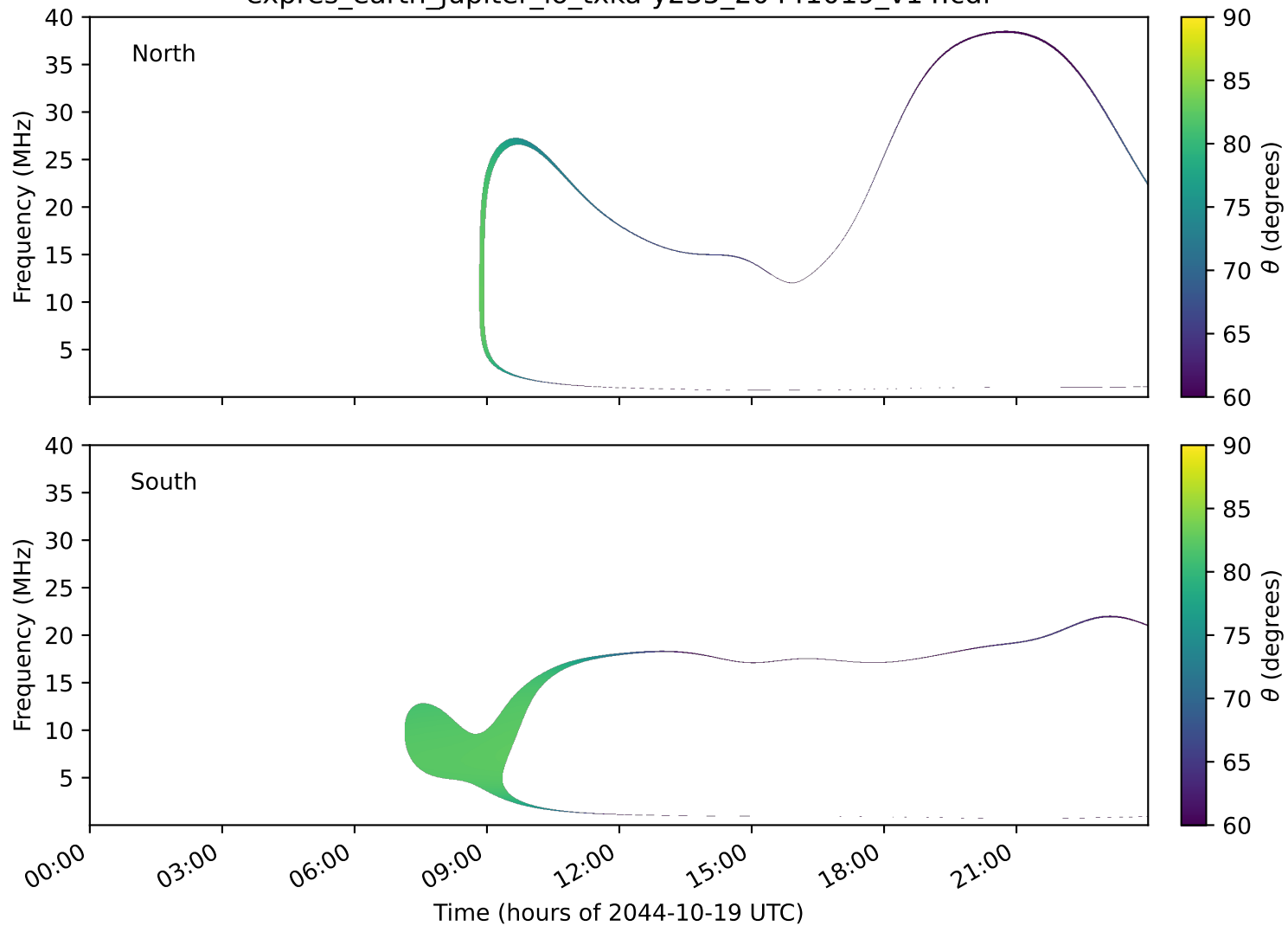
expres_earth_jupiter_io_txka-y235_20441019_v14.cdf
