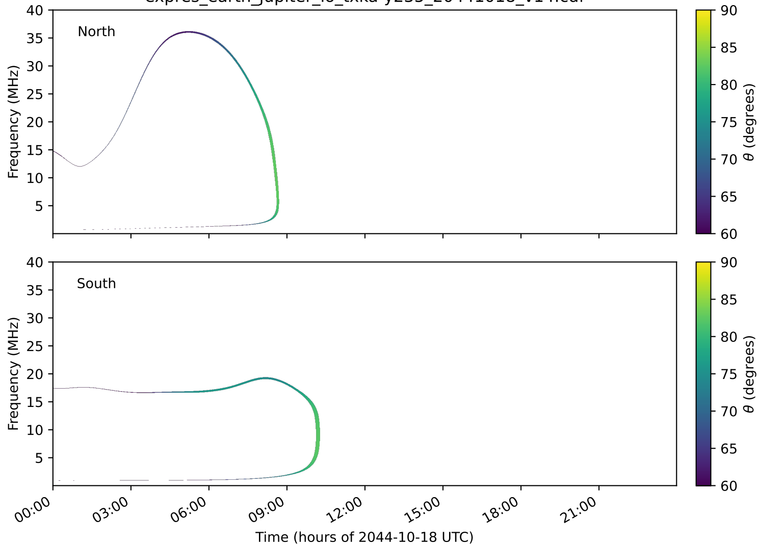
expres_earth_jupiter_io_txka-y235_20441018_v14.cdf
