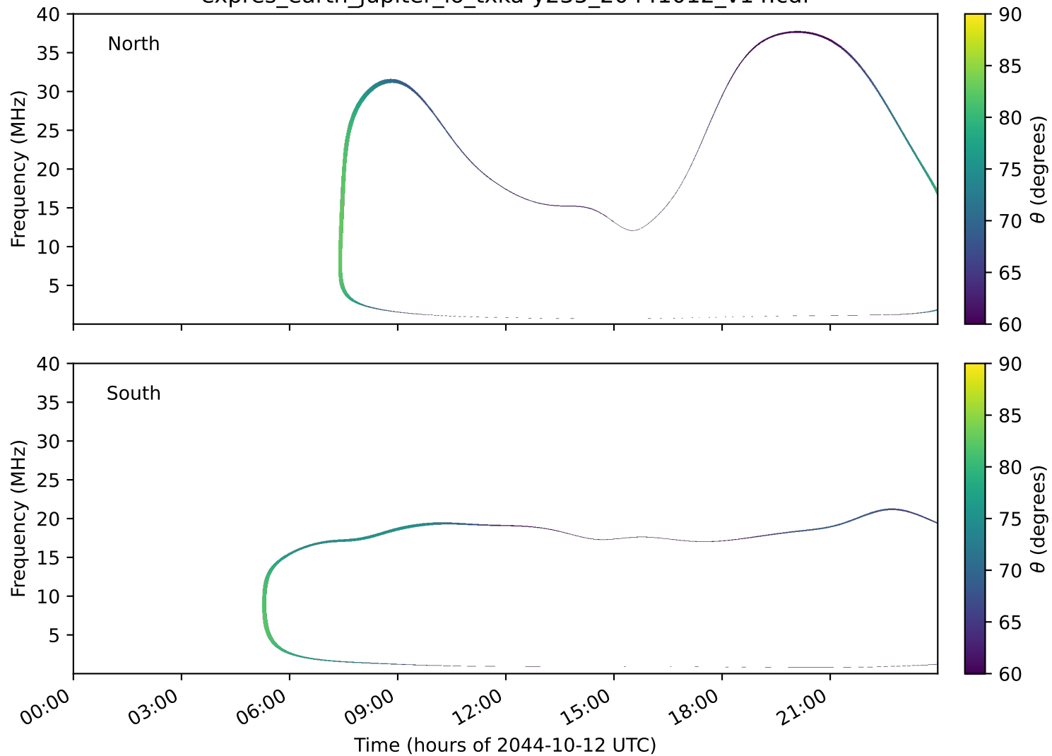
expres_earth_jupiter_io_txka-y235_20441012_v14.cdf
