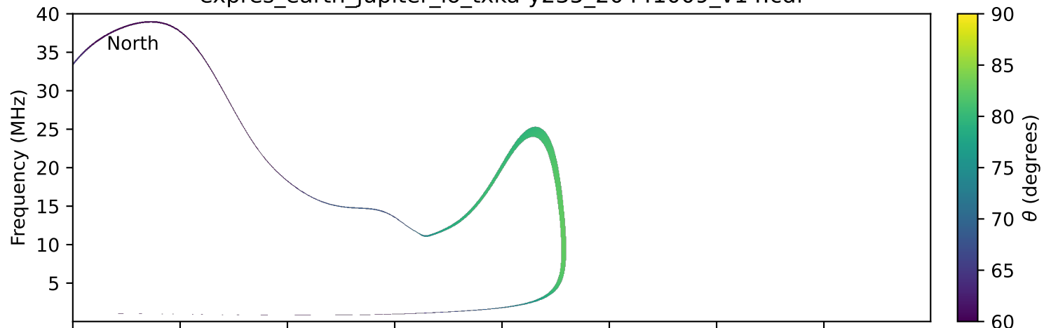
expres_earth_jupiter_io_txka-y235_20441009_v14.cdf
