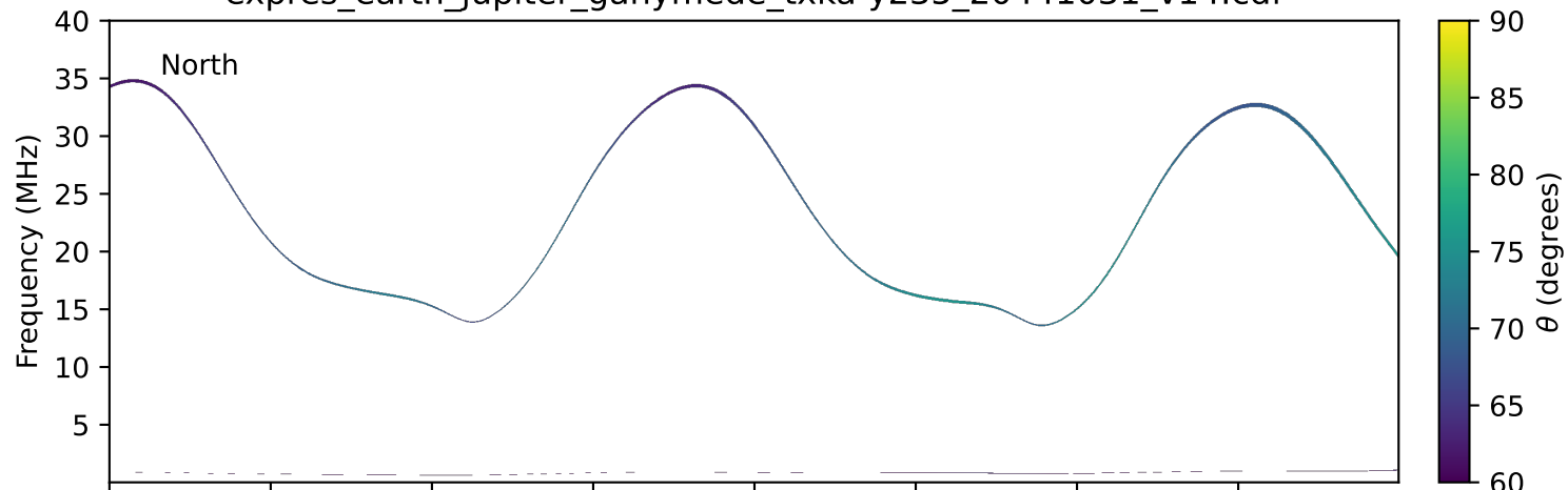
expres_earth_jupiter_ganymede_txka-y235_20441031_v14.cdf
