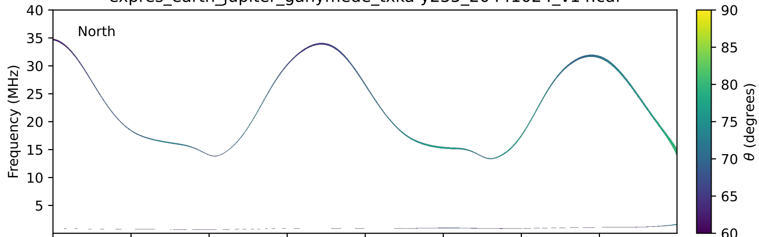
expres_earth_jupiter_ganymede_txka-y235_20441024_v14.cdf
