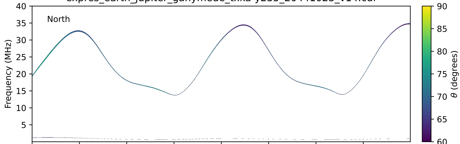
expres_earth_jupiter_ganymede_txka-y235_20441023_v14.cdf
