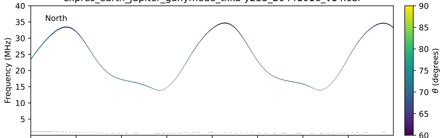
expres_earth_jupiter_ganymede_txka-y235_20441016_v14.cdf
