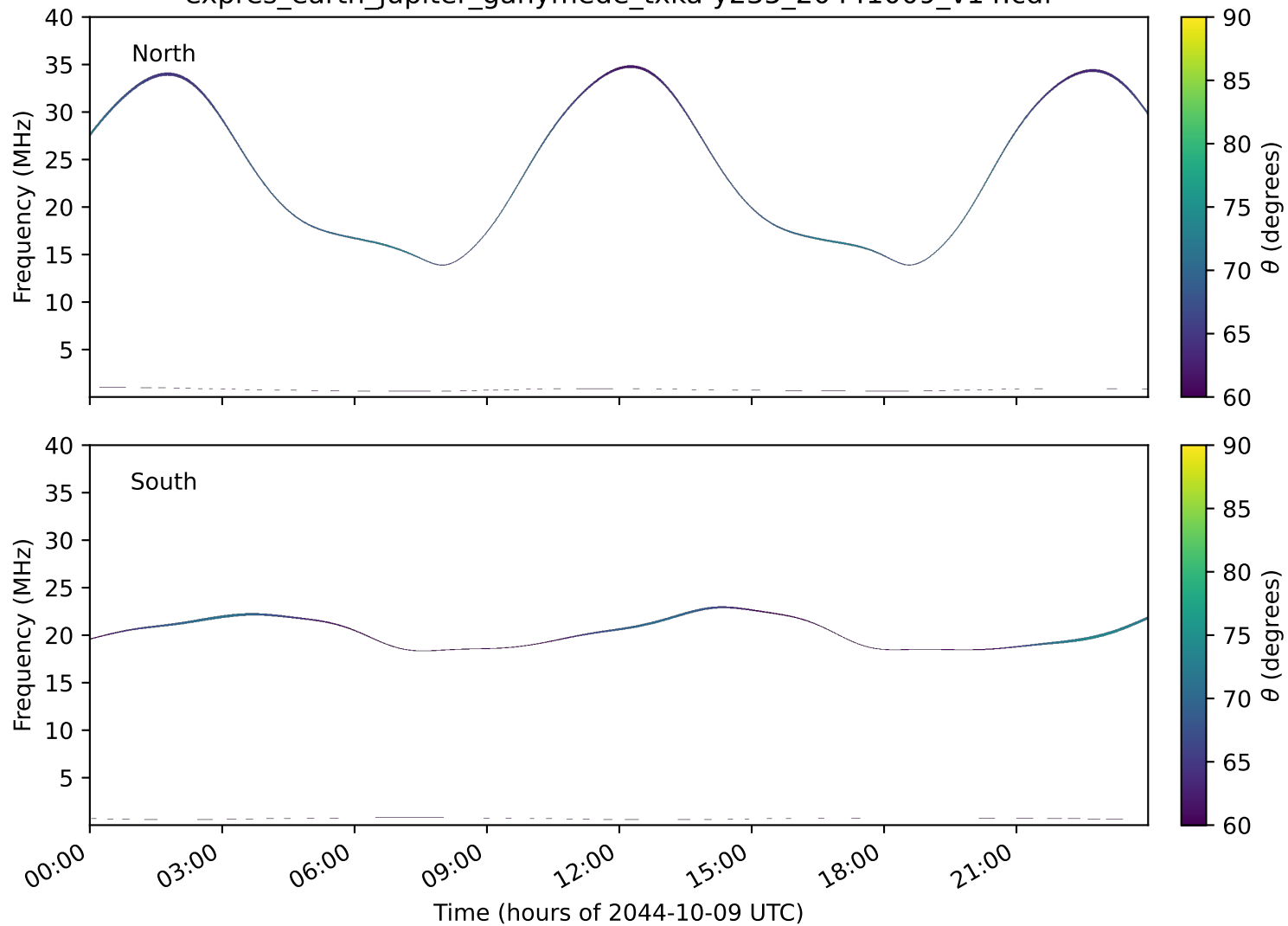
expres_earth_jupiter_ganymede_txka-y235_20441009_v14.cdf
