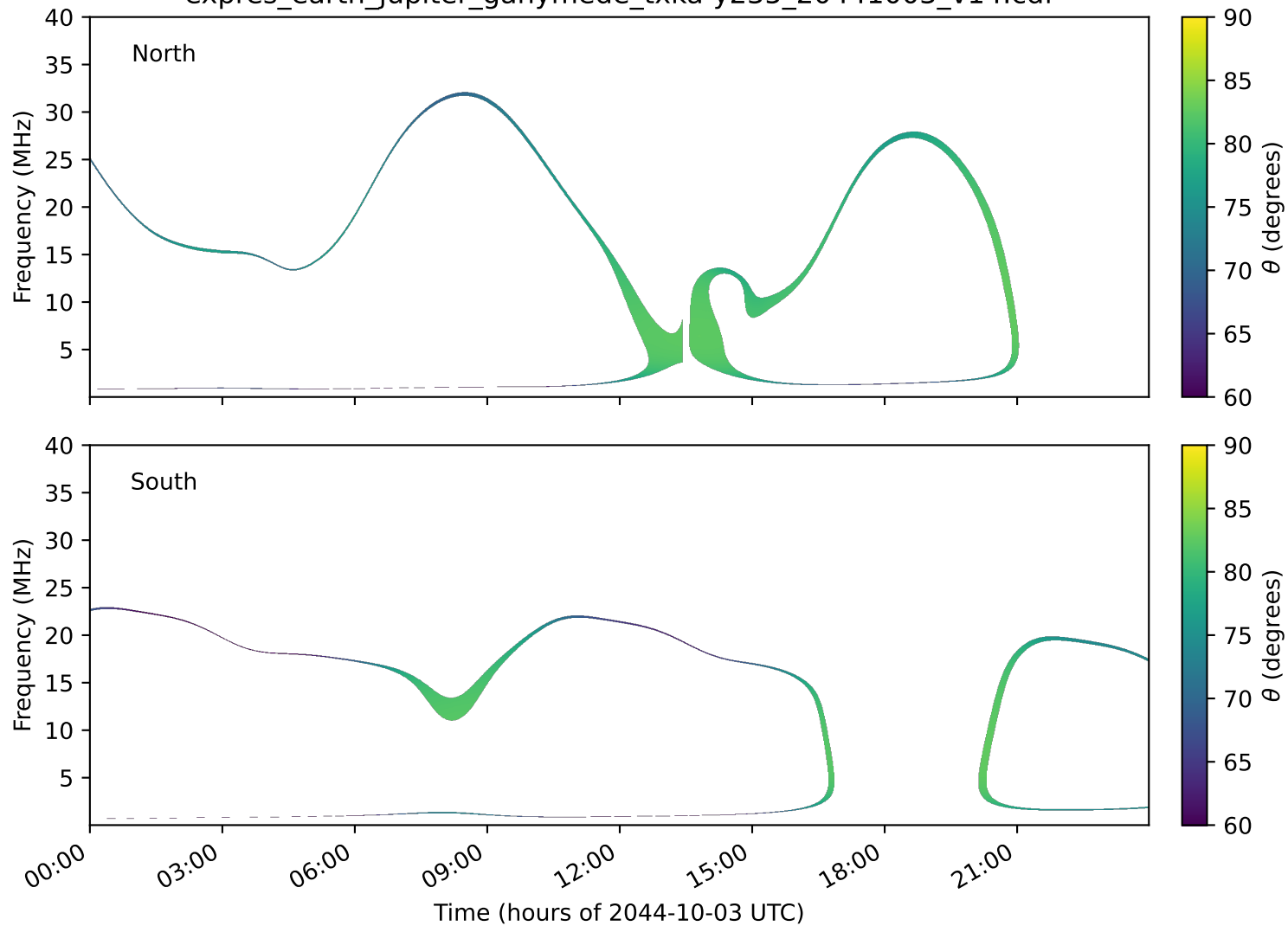
expres_earth_jupiter_ganymede_txka-y235_20441003_v14.cdf
