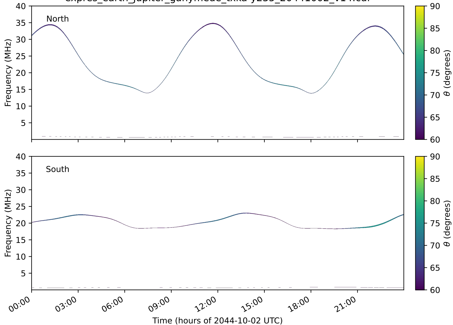
expres_earth_jupiter_ganymede_txka-y235_20441002_v14.cdf
