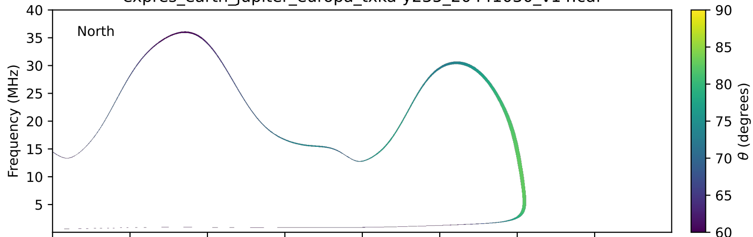
expres_earth_jupiter_europa_txka-y235_20441030_v14.cdf
