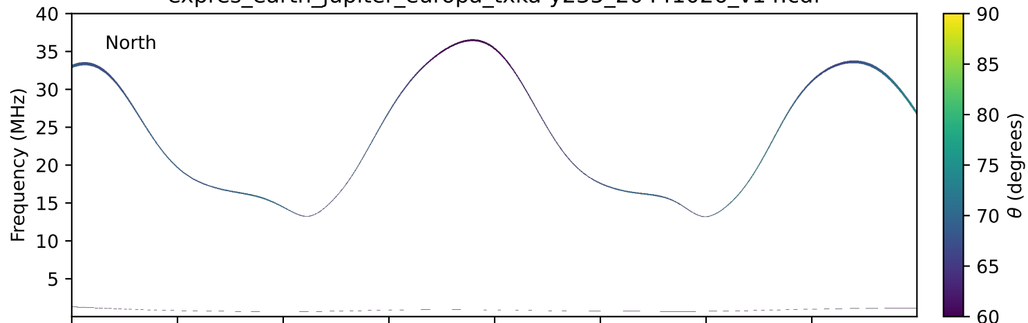
expres_earth_jupiter_europa_txka-y235_20441026_v14.cdf
