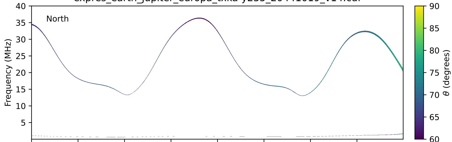
expres_earth_jupiter_europa_txka-y235_20441019_v14.cdf
