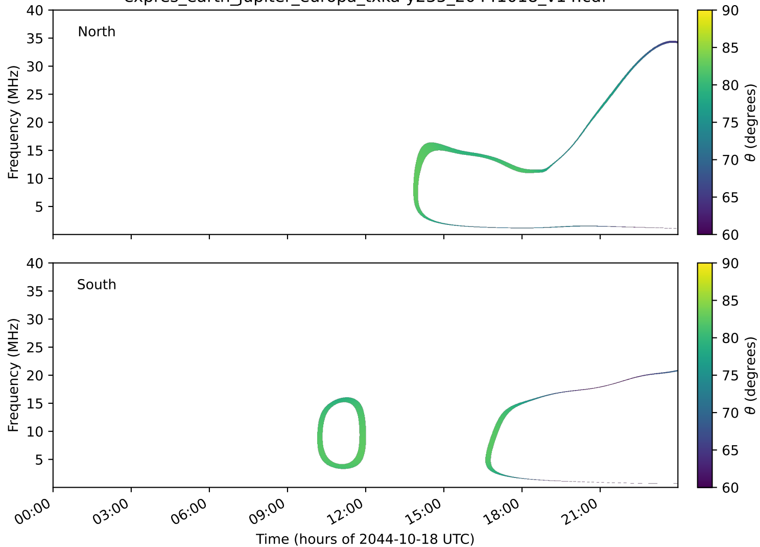
expres_earth_jupiter_europa_txka-y235_20441018_v14.cdf
