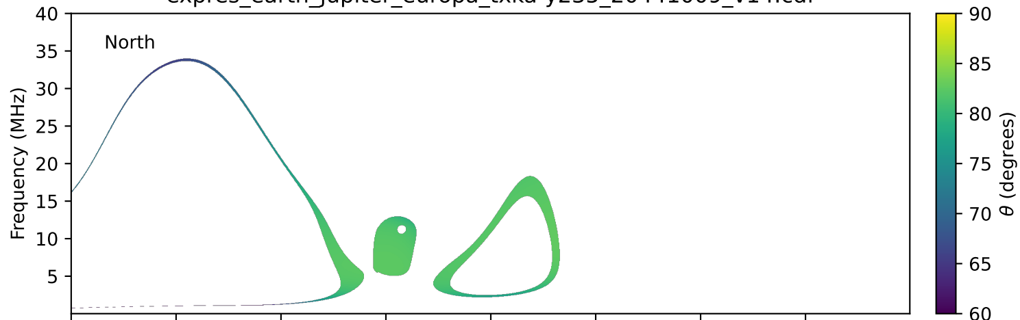
expres_earth_jupiter_europa_txka-y235_20441009_v14.cdf
