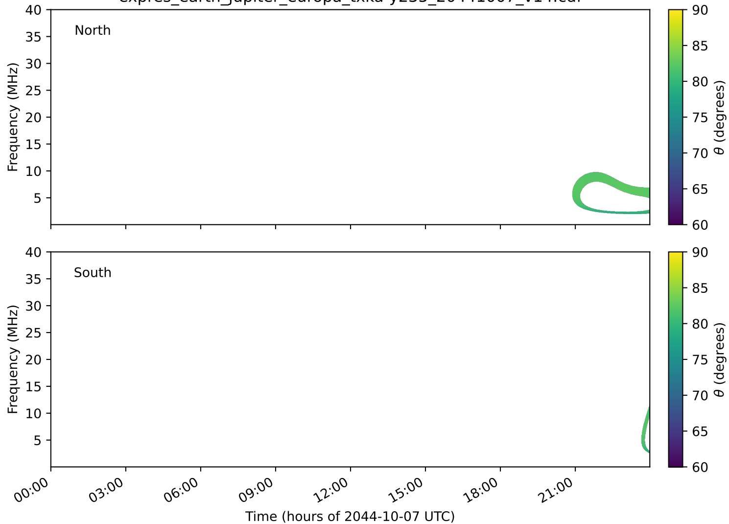
expres_earth_jupiter_europa_txka-y235_20441007_v14.cdf
