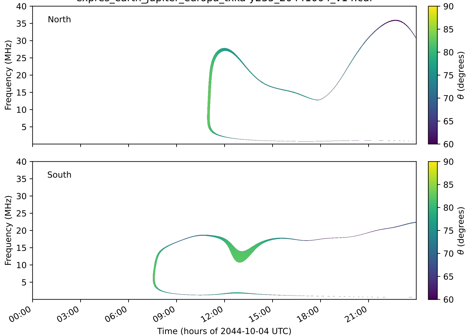
expres_earth_jupiter_europa_txka-y235_20441004_v14.cdf
